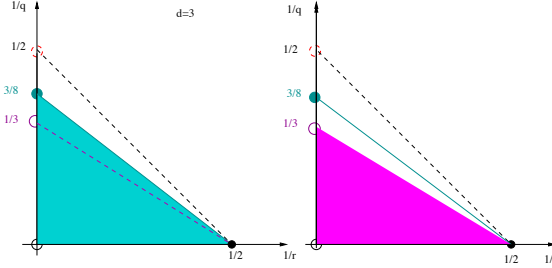
FIG. 4. Improved range of indices for which the Strichartz estimates hold for d = 3
