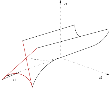
FIG. 7. The caustic for the swallowtail catastrophe.
