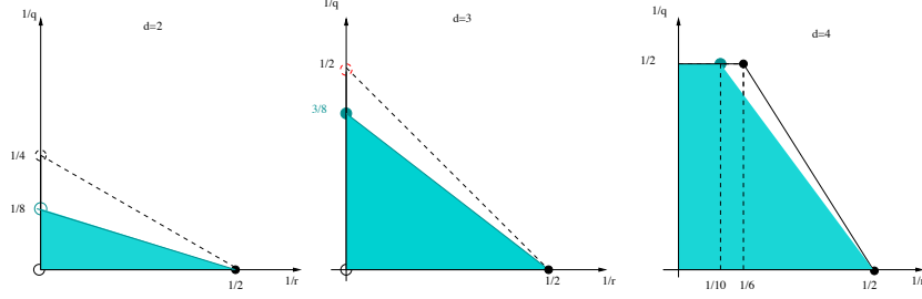
FIG. 3. Scale-invariant Strichartz estimates obtained from Theorem 2.9
