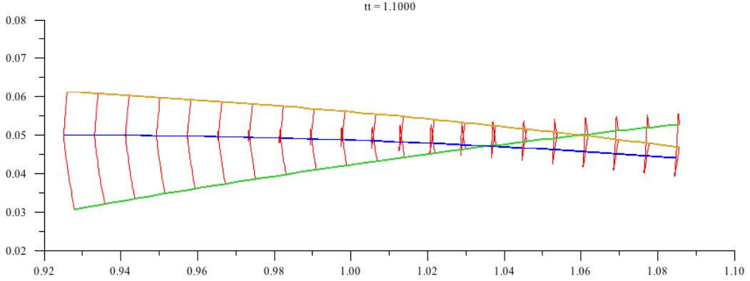
FIG. 9. The formation of a swallowtail singularity just after the first reflection (zoomed image)
