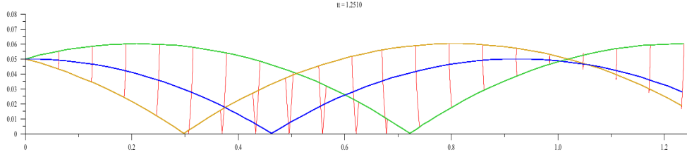
FIG. 8. Propagation of the wavefront
