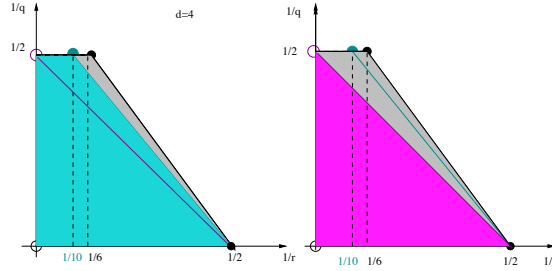
FIG. 5. Improved range of indices for which the Strichartz estimates hold for d = 4
