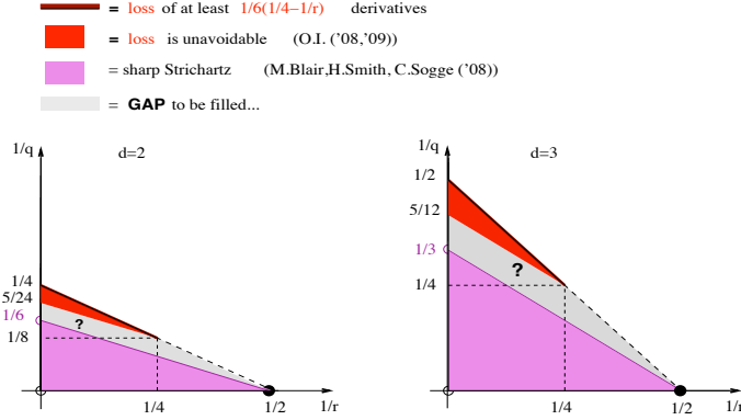
FIG. 2. Counterexample to the Strichartz estimates inside a bounded domain [8, 9]
