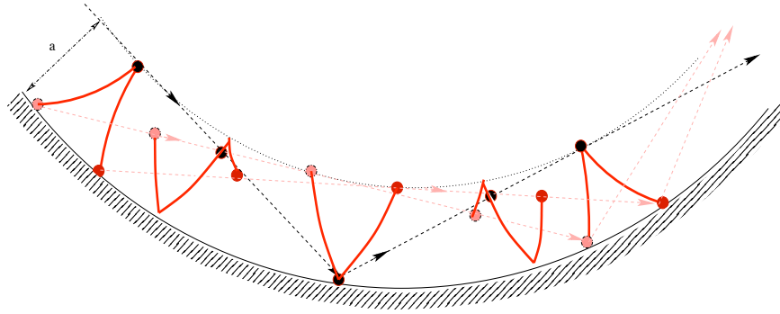
FIG. 6. Propagation of the cusp : preserving ray optics picture requires a > h^{1/2}
