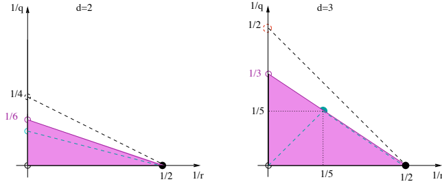
FIG. 1. Scale invariant Strichartz estimates obtained by [1] for d = 2, 3
